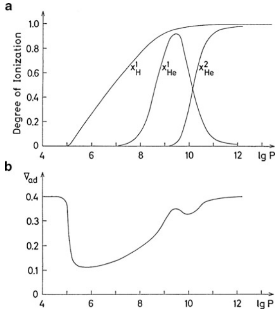
Fig. 14.1 Ionization in the outer layers of the Sun. (a) Degrees of ionization of hydrogen and helium. (b) The influence of ionization on \nabla_{\text{ad}}
