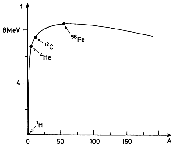
Fig. 18.1 A smoothed run of the fractional binding energy per nucleon, f = E_B/A , for stable nuclei, over the atomic mass number A . The curve is smoothed over the wiggles which are due to the nuclear shell structure and pair effects
