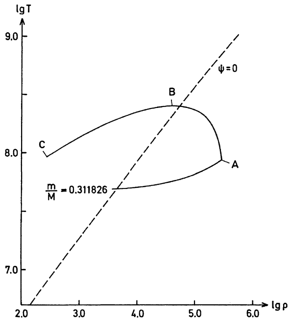
Fig. 33.8 Temperature T (in K) versus density \rho (in \text{g cm}^{-3} ) for the mass shell at which helium ignites in the 1.3M_{\odot} model. The letters A–C refer to the corresponding evolutionary states in Figs. 33.3 and 33.4. The dashed line (degeneracy parameter \psi = 0 for \mu_e = 2 ) roughly separates the regimes of degeneracy and non-degeneracy of the electron gas (After Thomas 1967)
