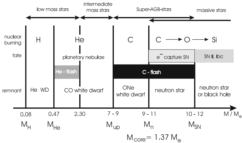
Fig. 34.10 Transition masses between different evolutionary paths for stars, and their final fate. M_{\text{H}} , M_{\text{He}} , M_{\text{up}} , M_{\text{n}} , and M_{\text{SN}} correspond to the minimum initial stellar mass for hydrogen, helium, and carbon ignition, the formation of a neutron star, and for stars undergoing a type II supernova explosion. The final fate of the star and its remnant are indicated for each mass range. Note that these mass limits depend crucially on the initial composition and on the detailed computations (After Siess 2006b )
