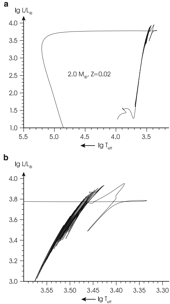
Fig. 34.8 (a) Evolution of a star of 2 M_{\odot} and Z = 0.02 from the ZAMS to the white-dwarf cooling stage (Weiss and Ferguson 2009). (b) Detail view of the TP-AGB phase, with 15 TPs, the last one leading to an excursion to very low T_{\text{eff}} , the final expulsion of the stellar envelope, and the beginning of the post-AGB transition to hot T_{\text{eff}} at nearly constant L . For details about the calculations, see text
