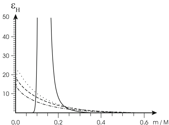
Fig. 30.2 Profiles of nuclear energy production \varepsilon_{\text{H}} from hydrogen burning (in erg/gs) for some of the models for which hydrogen profiles are shown in Fig. 30.1. These are the ones at the very beginning of hydrogen burning ( dash-dotted line ) and at ages of 6.2 ( dashed ), 8.2 ( dotted ), and 11.2 \times 10^9 years ( solid line ). The maximum energy generation rate in this latter model is 170 erg/gs
