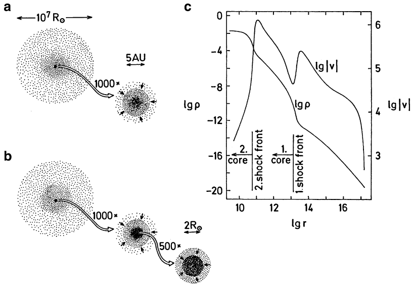
Fig. 27.2 The collapse of a gas cloud of 1M_\odot . (a) After about 1.3 \times 10^{13} s, the cloud has formed an optically thick core. The collapse is stopped there, and a shock front develops at the interface between the core, which is in hydrostatic equilibrium, and the still freely falling envelope. (b) When the core has become dynamically unstable owing to dissociation of \text{H}_2 , a second collapse occurs within the core, forming a second shock front at much smaller r . (c) Schematic plot of the absolute value of the velocity v (in \text{cm s}^{-1} ) and the density \rho (in \text{g cm}^{-3} ) against r (in cm), for a time shortly after the formation of a second core within the first one. The regions of the shock fronts are characterized by steep (positive) slopes in the velocity curve
