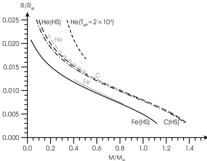
Fig. 37.4 R – M relation obtained from numerical white dwarf models. For comparison, the relations by Hamada and Salpeter (1961) for white dwarfs consisting of pure He, C, or Fe are repeated ( black lines , indicated by “HS” following the element label). The numerical results were obtained for white dwarfs with an effective temperature of 4,000–5,000 K. These are the shorter grey lines with the same line style as the HS-curves. The computations were restricted to a narrow mass range resulting from realistic previous stellar evolution models. The dashed black line with the label “He ( T_{\text{eff}} = 2 \times 10^4 )” is for a white dwarf with this effective temperature (data courtesy L. Althaus, after Panei et al. 2000)
