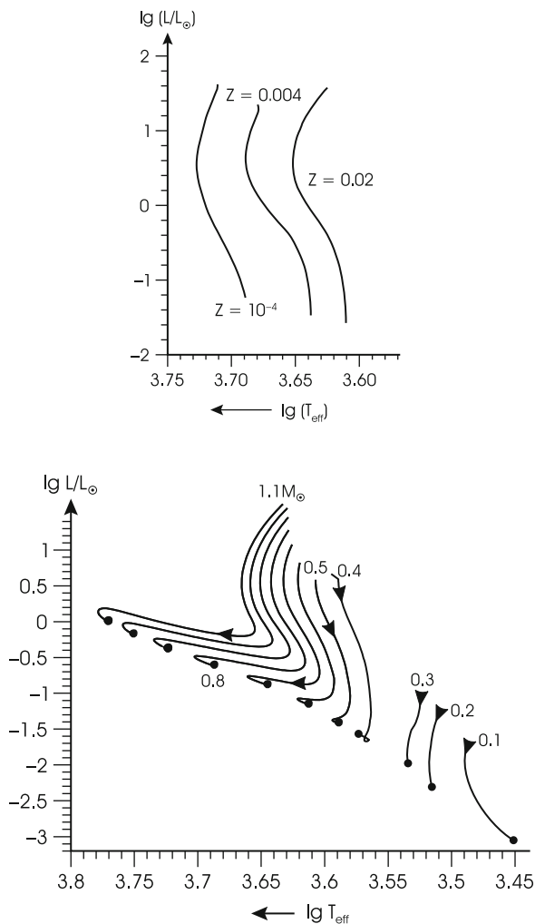
Fig. 24.3 Top: The position of Hayashi lines for stars of M = 0.8 M_{\odot} but different composition. The helium content is always 0.245, while Z varies from 10^{-4} to 0.02. Bottom: Pre-main-sequence evolution along the Hayashi line to the zero-age main sequence for stars between 0.1 and 1.1 M_{\odot} and a solar-like composition (Data courtesy S. Cassisi)
