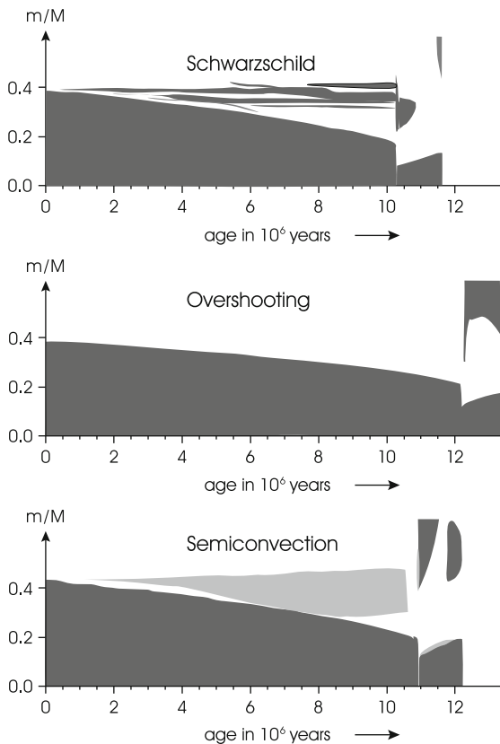
Fig. 30.12. Convective and semiconvective regions in a star of 15 M_{\odot} for three different treatments of convection. The top figure shows fully convective regions (dark grey) if the Schwarzschild criterion is applied. The bottom panel shows the result if the Ledoux criterion is used, and slow semiconvective mixing is done according to the diffusive approach by Langer et al. (1985) ; with the free parameter in this description set to 0.1). Semiconvective regions are indicated by light grey. The central panel finally shows the case with overshooting considered as a diffusive process according to (30.9), with f_{ov} = 0.02 . Note that only the convective core ( \nabla_{rad} \geq \nabla_{ad} ) is shown; the region of overshooting, which extends over more than 5 % of the mass, is not visible in this figure (but see Fig. 30.10)
