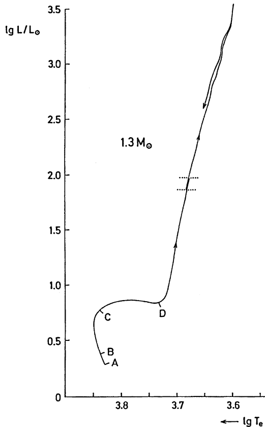
Fig. 33.3 The evolutionary track of a star of 1.3M_{\odot} with the initial composition X_{\text{H}} = 0.9 , X_{\text{He}} = 0.099 , Z = 1 - X_{\text{H}} - X_{\text{He}} = 0.001 as computed by Thomas (1967) . The letters A–D refer to the corresponding evolutionary states in Fig. 33.4 . The arrows indicate the direction of the evolution. This direction is reversed for a short period between the dotted horizontal lines . This transient drop in luminosity at about \lg L/L_{\odot} = 2 occurs when the hydrogen-burning shell crosses the chemical discontinuity left behind when the bottom of the outer convective zone moves outwards again in the mass scale after it has reached its deepest extension (see Fig. 33.4 )
