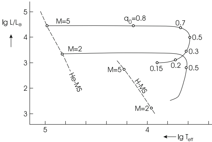
Fig. 23.6 The solid lines connect models of the same stellar mass M (in M_\odot ) on the different generalized main sequences of Fig. 23.5. Labels along the lines give the q_0 values of the generalized main sequences (After Lauterborn, Refsdal, Weigert, 1971a)
