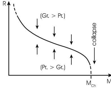
Fig. 37.1 Sketch of the classical mass–radius relation of white dwarfs according to Chandrasekhar’s theory (assuming that the pressure is provided only by an ideal, degenerate electron gas). The arrows indicate the direction into which a non-equilibrium configuration is pushed if the gravitational force (“Gr.”) is larger or smaller than the pressure gradient (“Pr.”). Corrections are necessary at both ends of the curve ( dashed )
