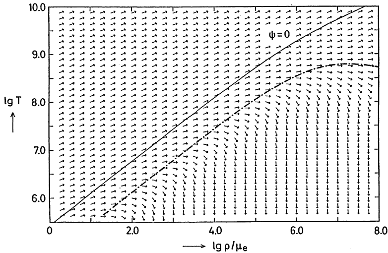
Fig. 28.1 The vector field given by (28.1) in a diagram showing the temperature T (in K) over the density \rho/\mu_e (in \text{g cm}^{-3} ). The arrows indicate the direction in which the centre of a homologously contracting star would evolve. In the upper-left part the equation of state is that of an ideal gas, and therefore the arrows have a slope of 1/3 . The thin solid line at which the degeneracy parameter \psi = 0 indicates roughly the transition from the ideal gas to degeneracy of the electrons. The critical line along which \alpha = 3/4 is dot-dashed . On this curve the arrows point horizontally while below it the arrows point downwards
