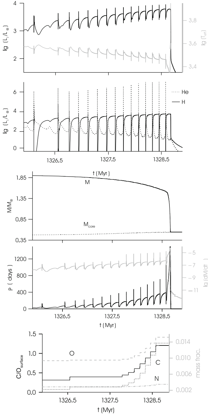
Fig. 34.9 Physical quantities during the TPs of the same model as in Fig. 34.8. The panels show, from top to bottom : total luminosity L ( left scale ) and T_{\text{eff}} ( right scale ); helium and hydrogen shell luminosity; total and C/O core mass; pulsation period ( left scale ) and mass loss rate ( right scale ); and finally C/O ratio at the surface ( left scale ) and C, N, and O mass fractions ( right scale )
