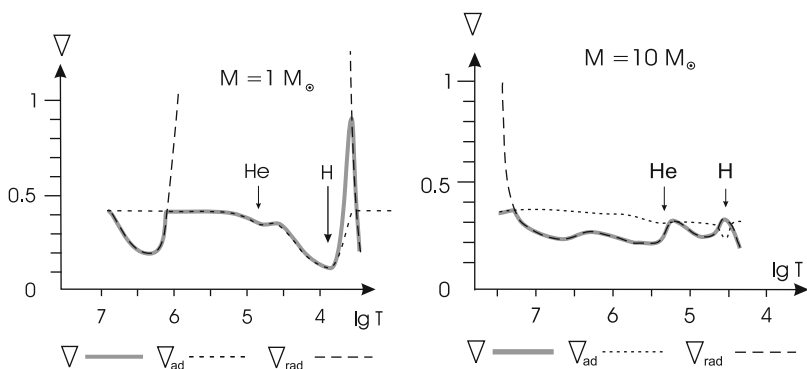
Fig. 22.8 The grey solid lines show the actual temperature gradient \nabla = d \ln T / d \ln P over the temperature T (in K) inside two zero-age main-sequence models of 1 M_{\odot} (left panel) and 10 M_{\odot} (right panel). The corresponding adiabatic gradients \nabla_{\text{ad}} (dotted lines) and radiative gradients \nabla_{\text{rad}} (dashed lines) are also plotted, and the location of the ionization zones of hydrogen and helium are indicated (arrows). The chemical composition of the models is the same as for those of Fig. 22.1
