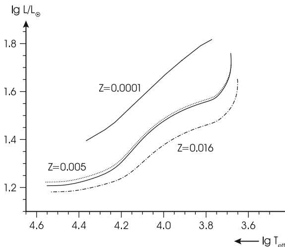
Fig. 33.11 Zero-age horizontal-branch (ZAHB) models for different compositions. The ZAHB brightness increases with decreasing metallicity, which is in this version Z = 0.016, 0.005 , and 0.0001 . The two lines for Z = 0.005 correspond to ages of 15 Gyr ( dotted ) and 5 Gyr ( solid )
