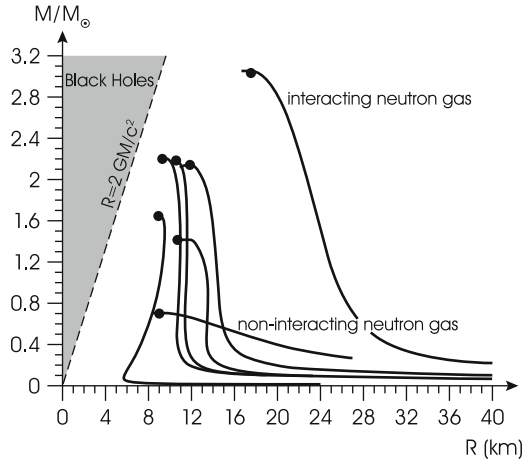
Fig. 38.1 The relation M against R of neutron-star models calculated using seven different equations of state. The maximum mass is indicated in each case by the solid dot . Two extreme assumptions are specifically indicated: a non-interacting neutron gas ( Oppenheimer and Volkoff 1939 ), which leads to an extremely soft equation of state and a very low maximum mass, and one where interactions are included and which leads to a maximum neutron star mass above 3M_{\odot} (After Fig. 10.3 in Weber et al. 2009 , where also details about the other five equations of state can be found)
