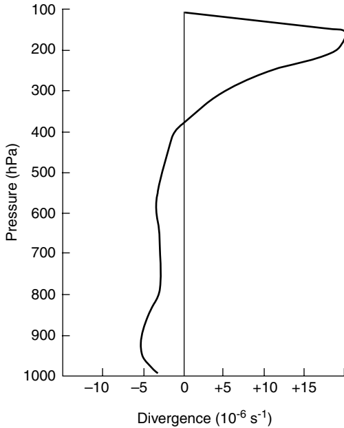
Fig. 11.5 Vertical profile of 4°-square area average divergence based on composites of many equatorial disturbances. (Adapted from Williams, 1971.)
